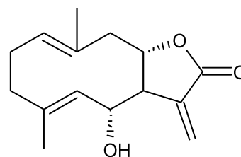
Deacetyl laurenobiolide
